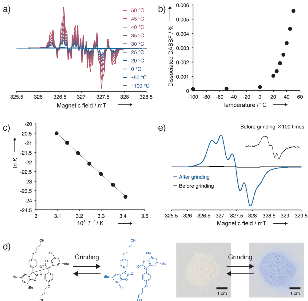
Figure 2. a) EPR spectra of a 100 mM solution of DABBF-diol in benzene in the temperature range from -100 to 50^\circ\text{C} . b) Percentage of dissociated DABBF-diol in benzene (100 mM) in the temperature range from -100 to 50^\circ\text{C} . c) van't Hoff plot for the disassociation of DABBF-diol in benzene (100 mM). d) Chemical structures, photographs, and e) EPR spectra of the powder of DABBF-diol before and after grinding at 25^\circ\text{C} in air.
